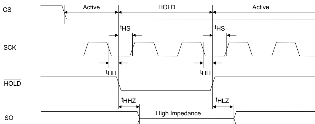
Figure 17 \overline{\text{HOLD}}
