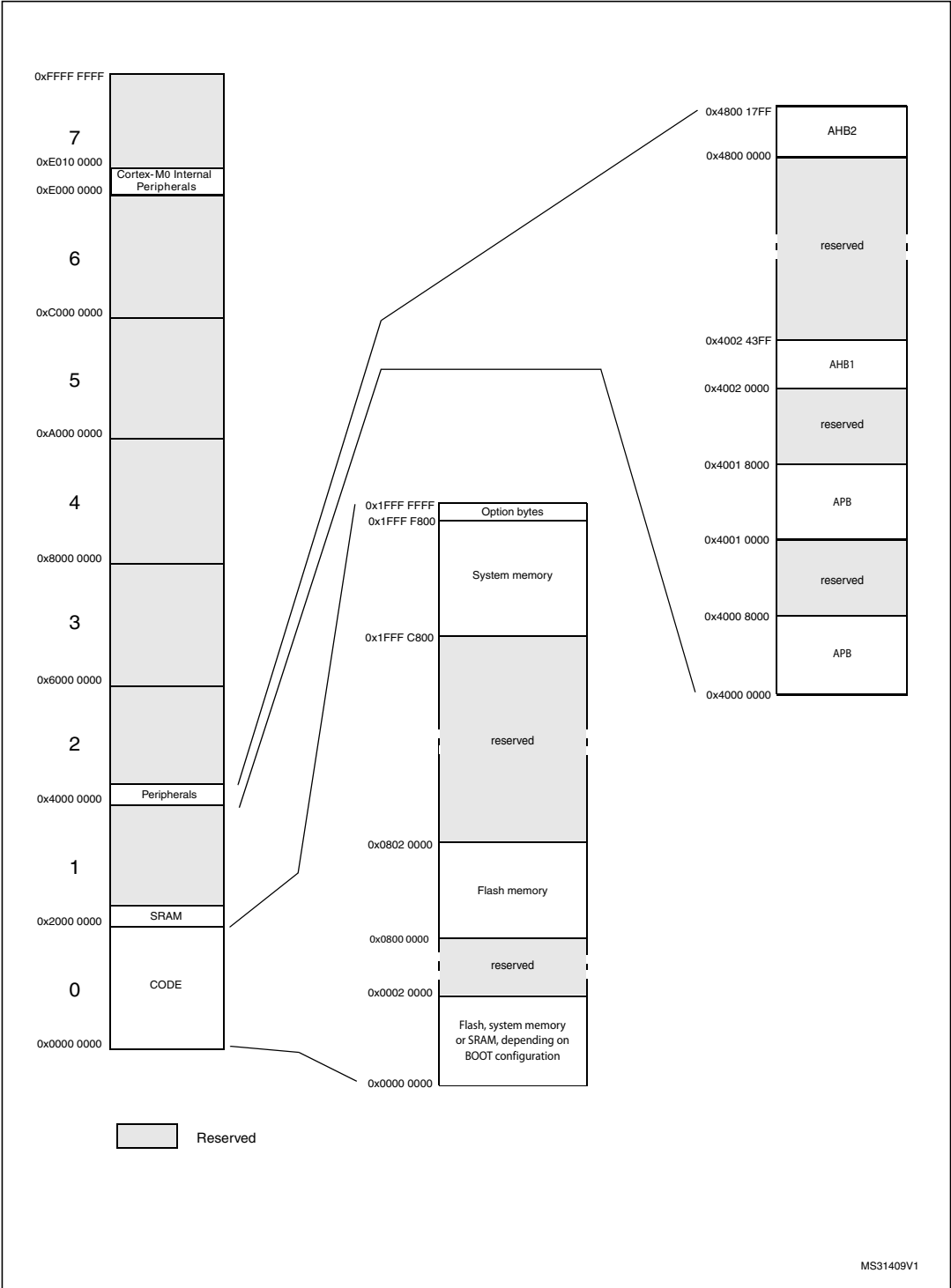
Figure 9. STM32F072xx memory map
