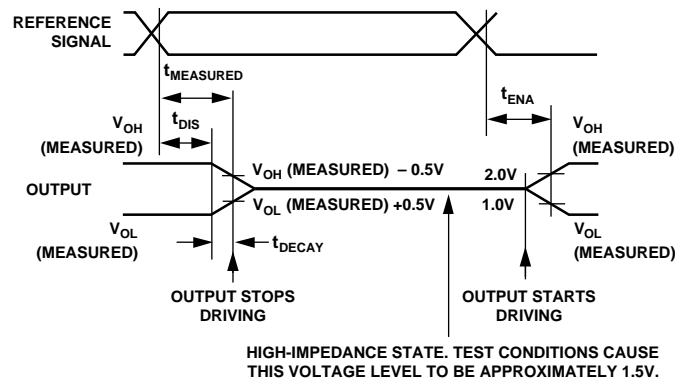
Figure 22. Output Enable/Disable
