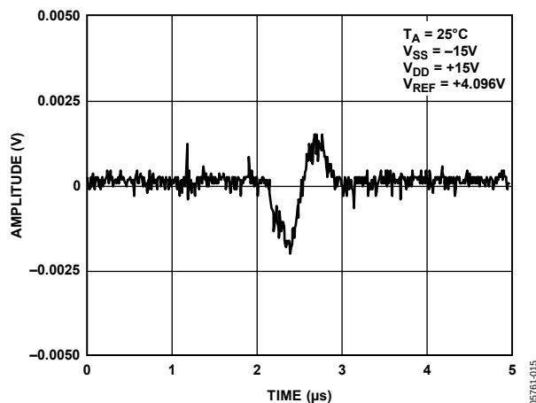
Figure 12. Digital Crosstalk
