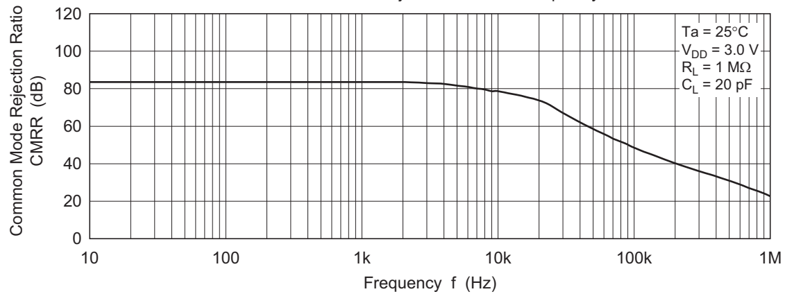
Figure 2-13. HA1630Q02 Common Mode Rejection Ratio vs. Frequency
