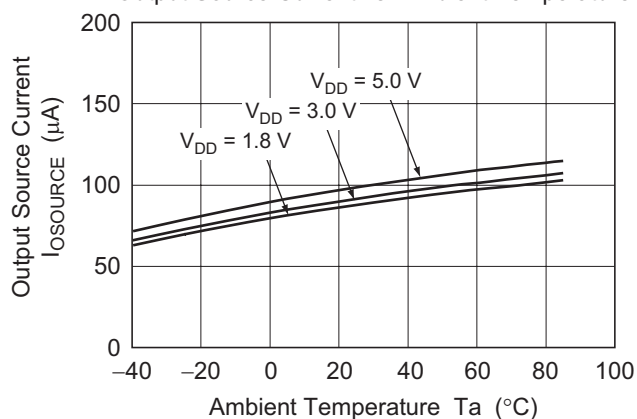
Figure 3-5. HA1630Q03 Output Source Current vs. Ambient Temperature
