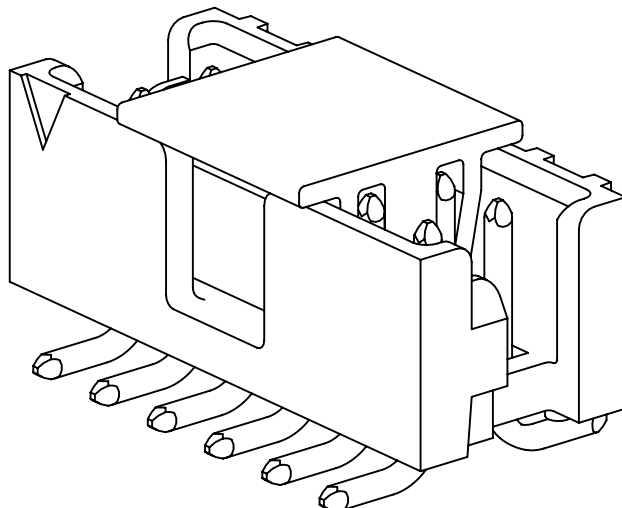
POLARIZATION SLOT SURFACE MOUNT HEADER 6-12 POSITIONS ONLY
