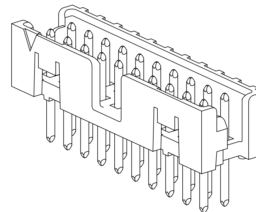
POLARIZATION SLOT AND DUAL FRICTION LATCHES THRU-HOLE VERTICAL HEADFE 14-50 POSITIONS
