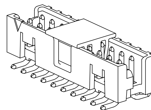
STANDARD LENGTH, POLARIZATION SLOT, DUAL FRICTION LATCHES, SURFACE MOUNT HEADER 14-50 POSITIONS
