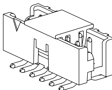
EXTENDED LENGTH, SINGLE FRICTION LATCH, SURFACE MOUNT HEADER 6-12 POSITIONS
