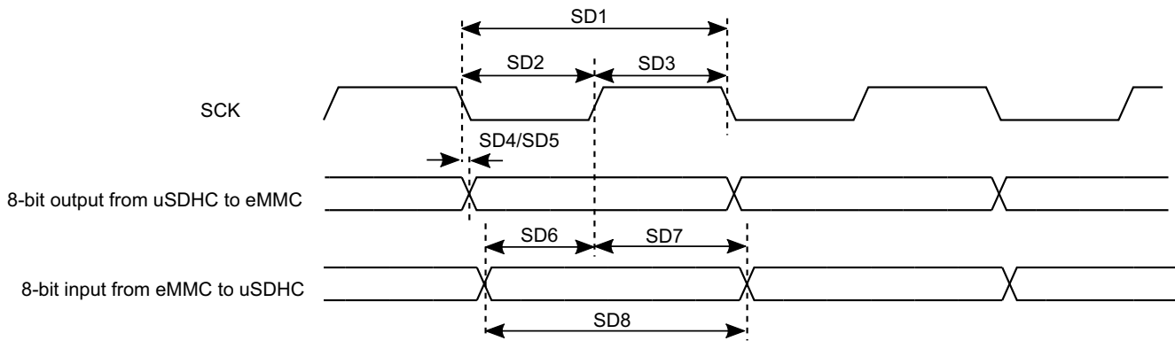
Figure 16. SDR50/SDR104 timing
