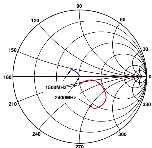
Figure 21. Output Impedance Smith Chart
