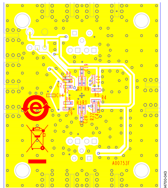
Figure 43. AD8341 Evaluation Board Bottom Layer
