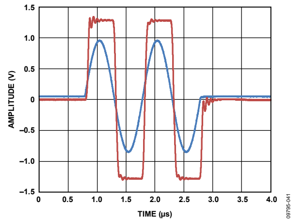
Figure 19. Overdrive Recovery
