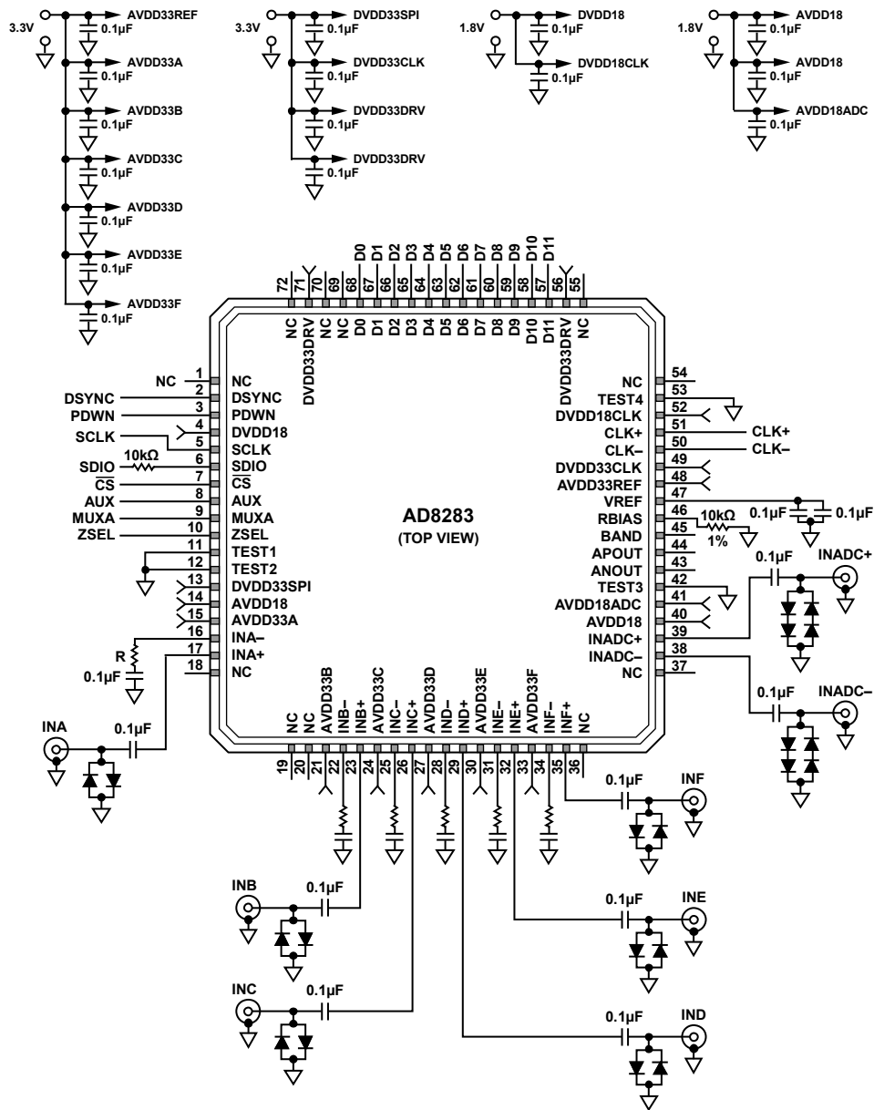
Figure 34. Single-Ended Inputs
