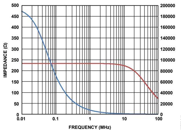
Figure 18. R_{IN} vs. Frequency
