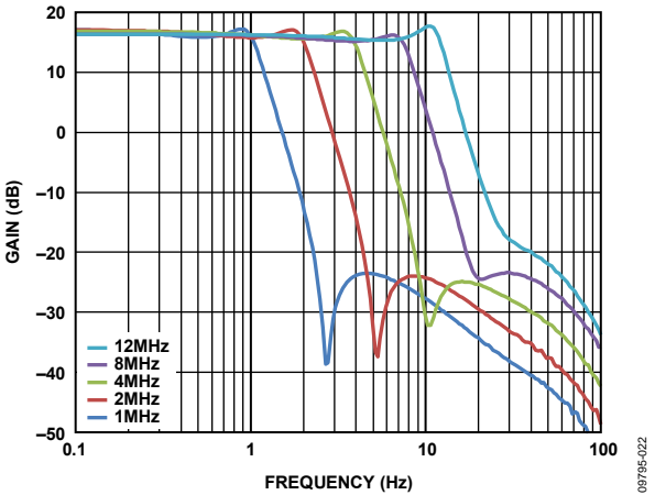
Figure 14. Filter Response
