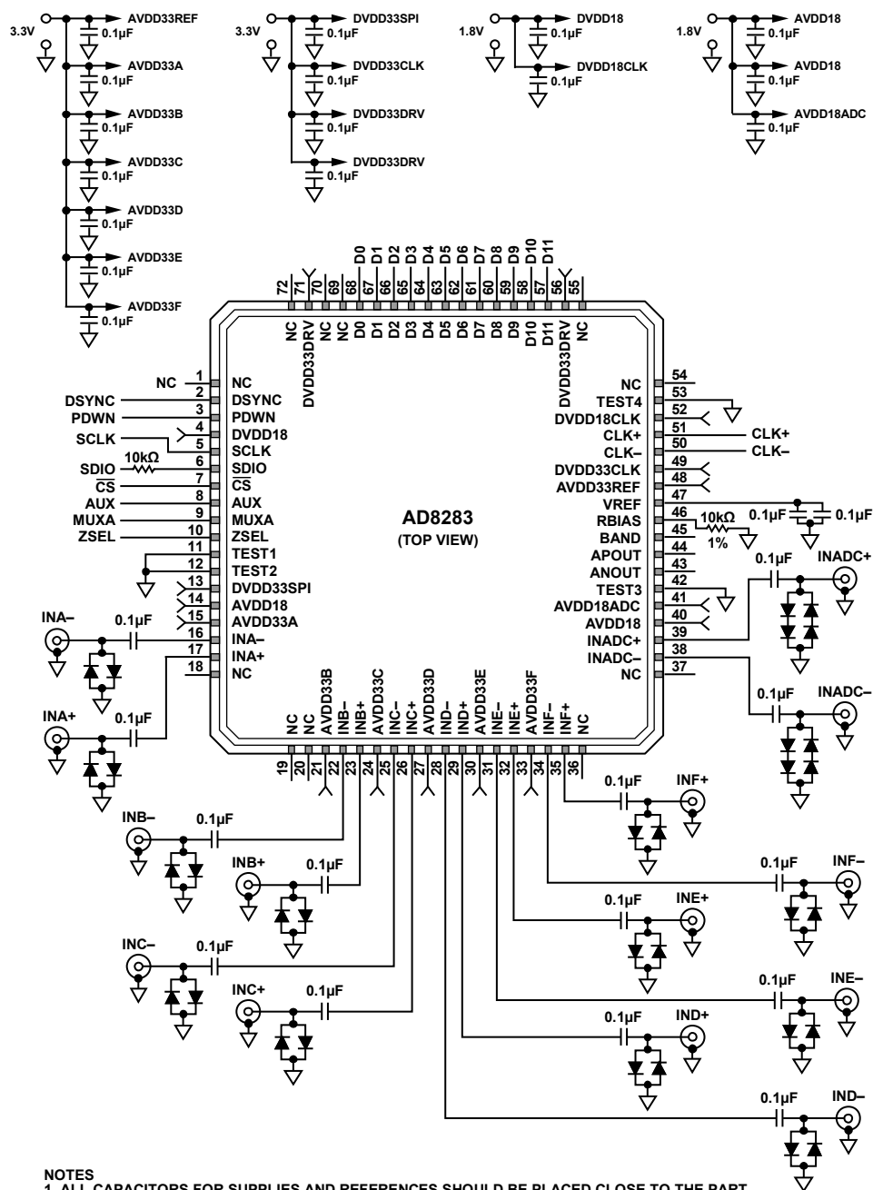
Figure 33. Differential Inputs
