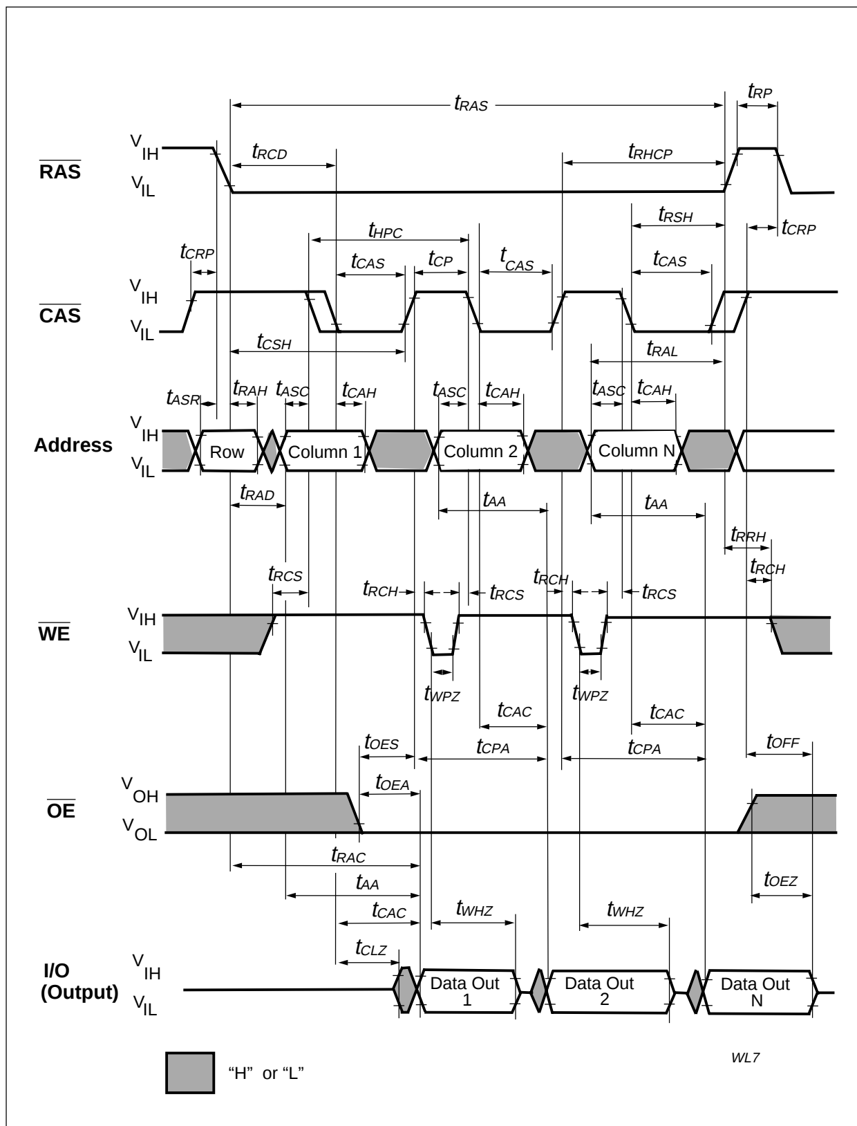
Hyper Page Mode (EDO) Read Cycle ( \overline{\text{WE}} Control)
