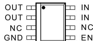
MIC5200-x.xBM (SOIC-8)
