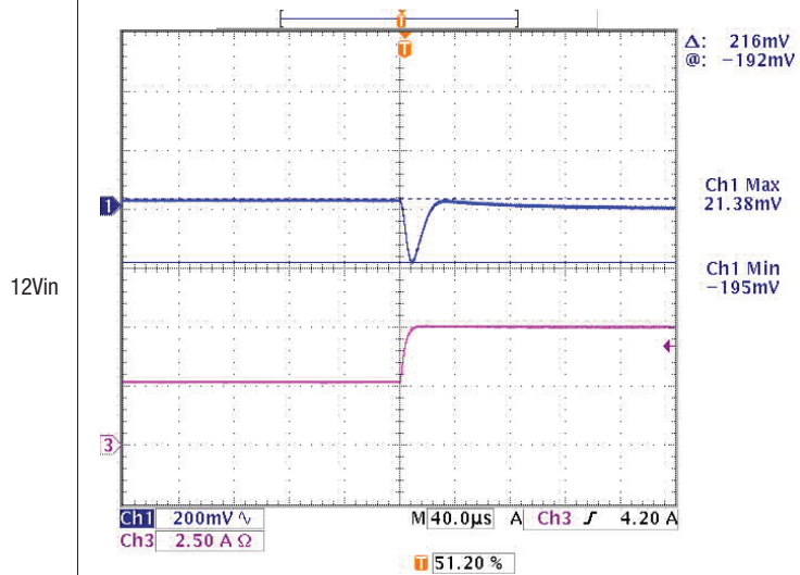
Step Load Transient Response (V in =12V, V out =5V, C load = 1 uF || 10 uF) Top trace=V out , Bottom trace=I out
