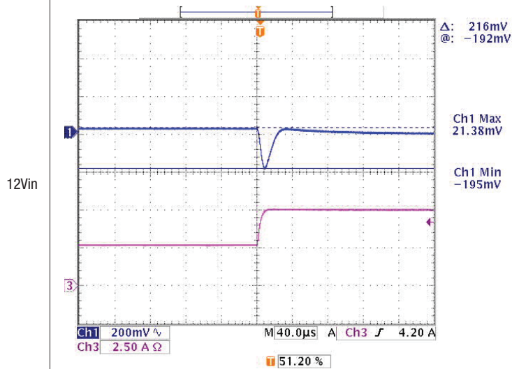
Step Load Transient Response (V IN =12V, V OUT =5V, C LOAD = 1 uF || 10 uF) Top trace=V out , Bottom trace=I out 2.5A → 5.0A
