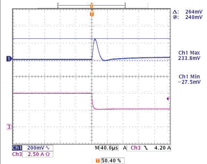
Step Load Transient Response (V in =12V, V out =5V, C load = 1 uF || 10 uF) Top trace=V out , Bottom trace=I out
