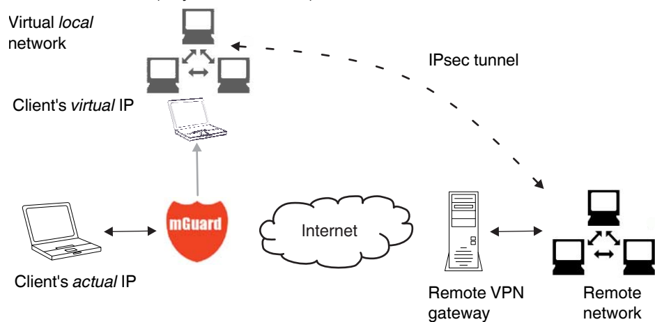
Figure 5-4 Virtual IP
