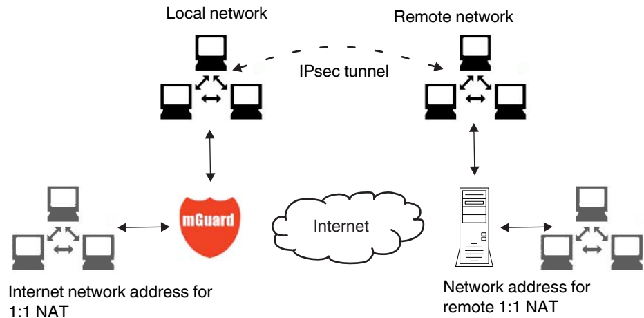
Figure 5-5 1:1 NAT
