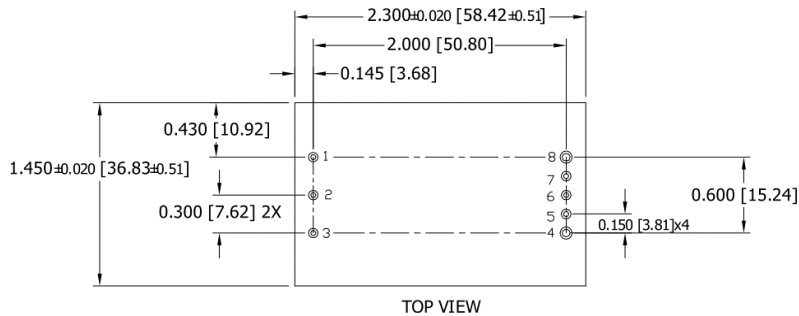
QM48T (Through-Hole)
