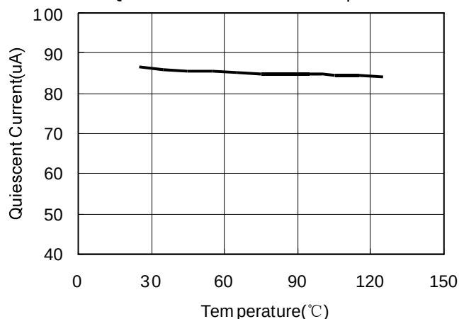
4. Quiescent Current vs Temperature
