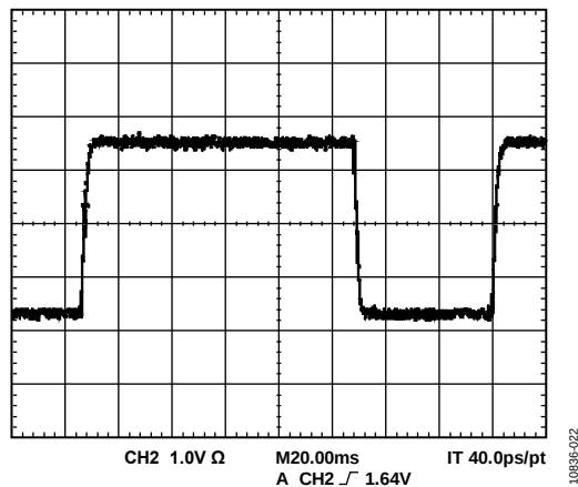
Figure 22. SYNC_OUT ( f_{\text{SYSCLK}}/384 )
