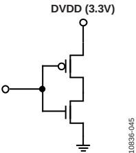
Figure 28. CMOS Input
