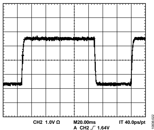
Figure 22. SYNC_OUT ( f_{\text{SYSCLK}}/384 )
