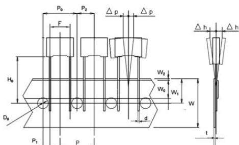
Lead Spacing 7.5 mm
