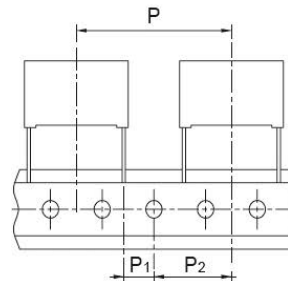
Lead Spacing 22.5 & 27.5
