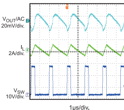
Steady State I_{OUT}=0A , Forced CCM Mode
