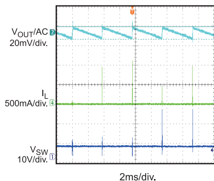
Steady State I_{OUT}=0A , AAM Mode
