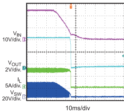
Shutdown Through V_{IN} I_{OUT}=7A
