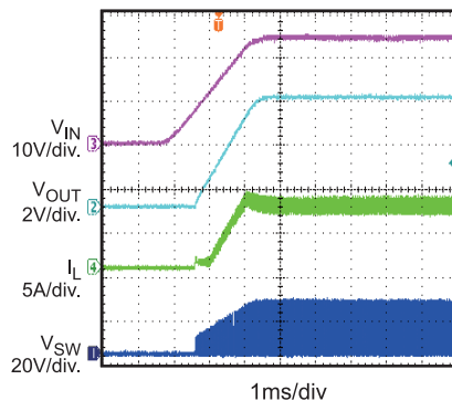
Start-Up Through V_{IN} I_{OUT}=7A
