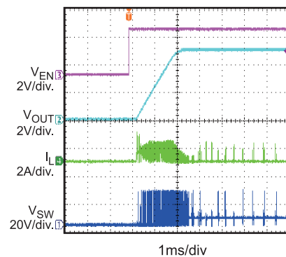
Start-Up Through EN/SYNC I_{OUT}=0A
