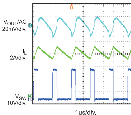
Steady State I_{OUT}=7A
