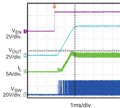
Start-Up Through EN/SYNC I_{OUT}=7A
