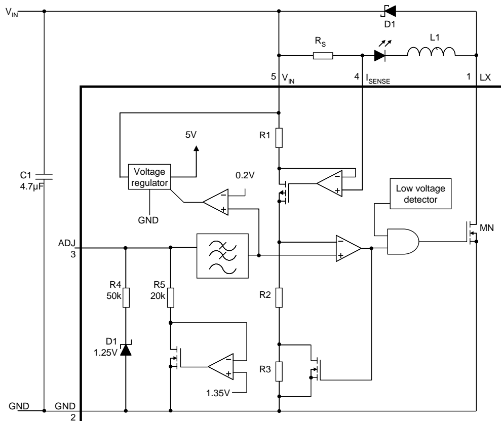
Figure 1. Block Diagram
