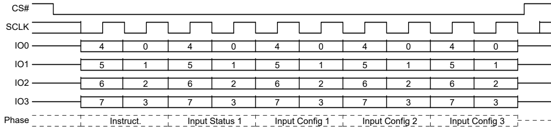
Figure 58. Write Register (WRR) Command Sequence QPI
