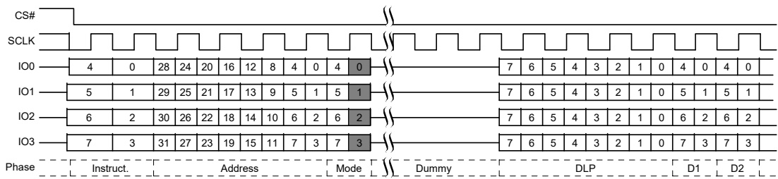
Figure 17. DDR Quad I/O Read Command QPI Mode
