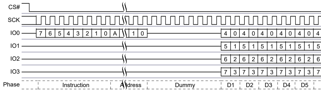
Figure 79. Quad Output Read Command Sequence
