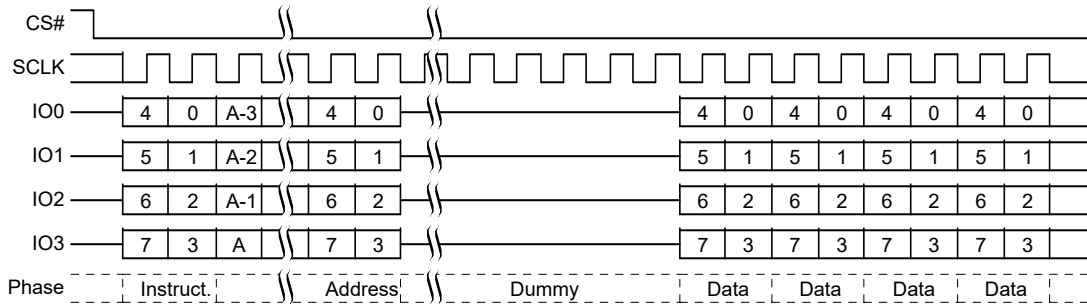
Figure 66. ECC Status Register Read QPI Mode, Command Sequence
