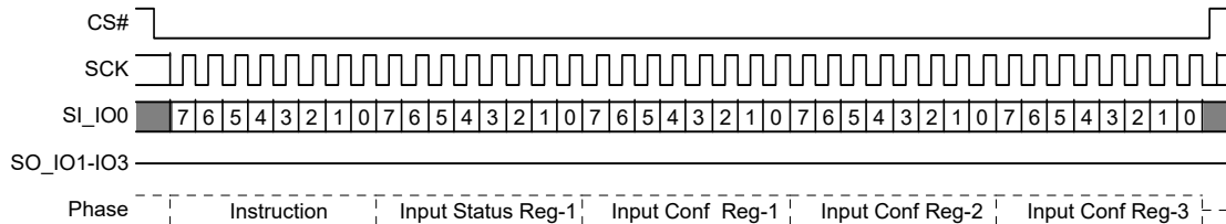
Figure 57. Write Register (WRR) Command Sequence
