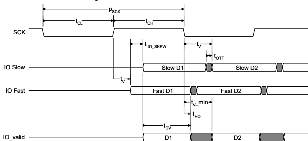
Figure 38. SPI DDR Data Valid Window
