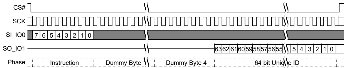
Figure 51. Read Unique ID (RUID) Command Sequence
