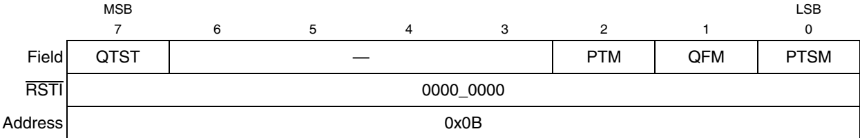
Figure 23-5. READI Mode Control (MC) Register
