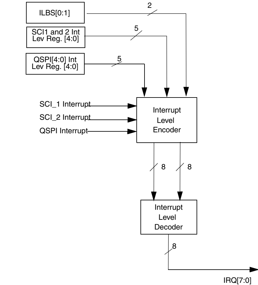
Figure 14-3. QSPI Interrupt Generation
