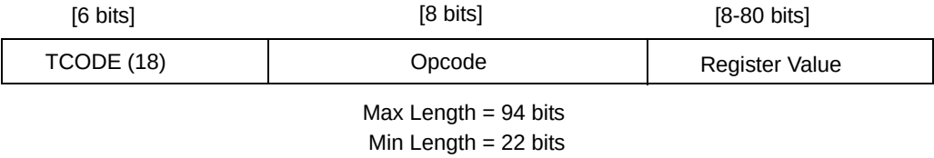
Figure 23-56. Write Register Message
