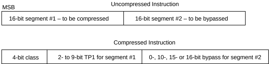
Figure A-9. CLASS_3 Instruction Layout
