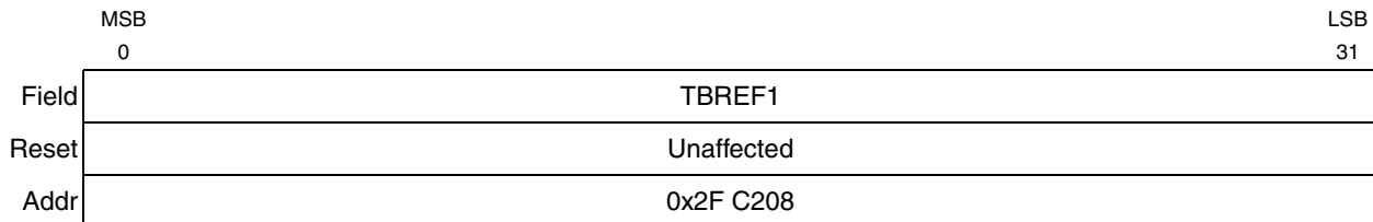
Figure 6-33. Time Base Reference Register 1 (TBREF1)
