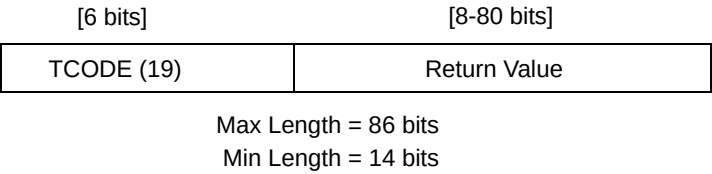
Figure 23-57. Read/Write Response Message
