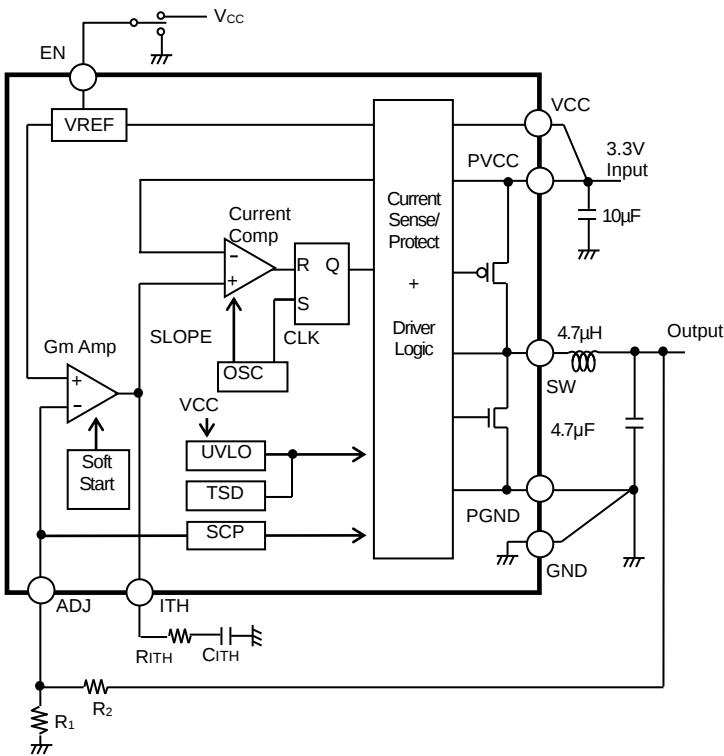
Figure 3. Block Diagram
