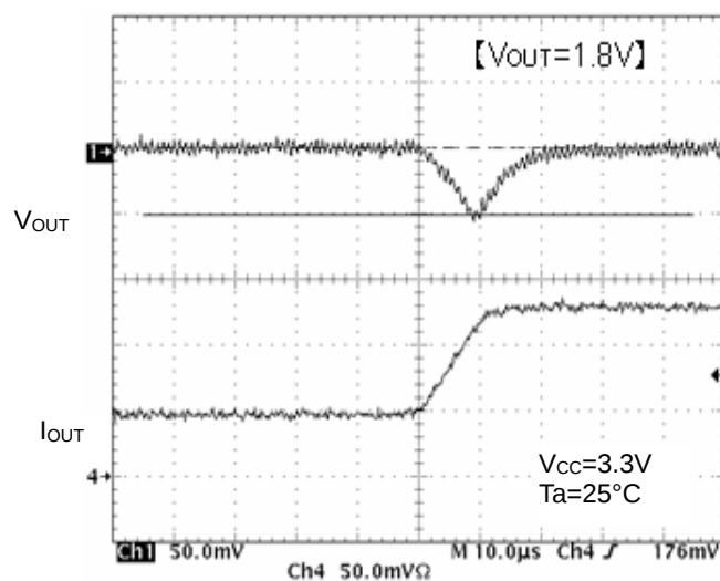
Figure 17. Transient Response ( I_o=50mA to 125mA, 10μs)
