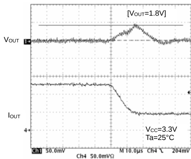
Figure 18. Transient Response ( I_o=125mA to 50mA, 10μs)
