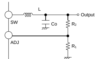
Figure 34. Determination of Output Voltage
