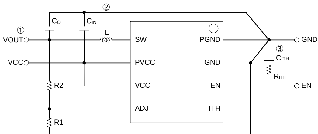
Figure 35. Layout Diagram
