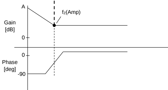
Figure 32. Error Amp Phase Compensation Characteristics
