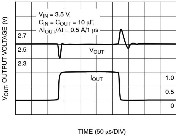
Figure 23. Load Transient ( V_{out} = 2.5\text{ V} )
