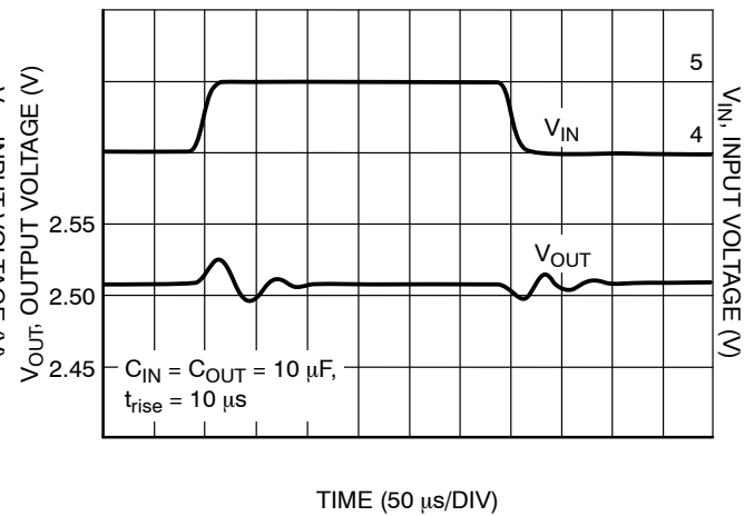
Figure 26. Line Transient ( V_{out} = 2.5 V )
