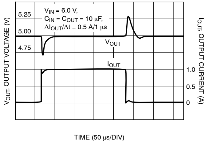
Figure 24. Load Transient ( V_{out} = 5.0 V )
