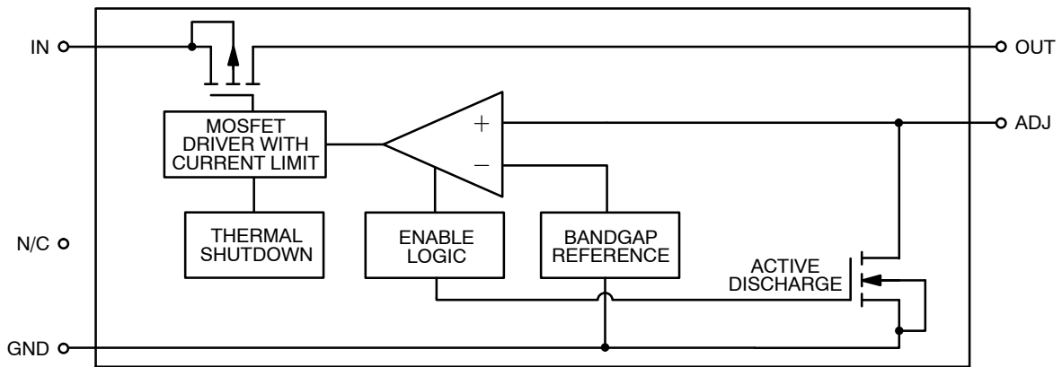
Figure 8. NCP690 Block Diagram (Adjustable Version)
