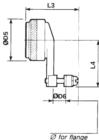
elbow cable clamp type 03
