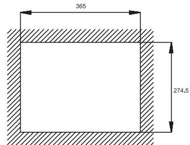
Panel Mount Cut-out (PPC-123)
