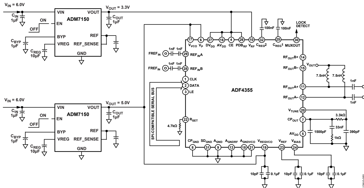
Figure 45. ADF4355 Power Supplies
