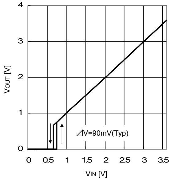
Figure.12 V IN -V OUT
