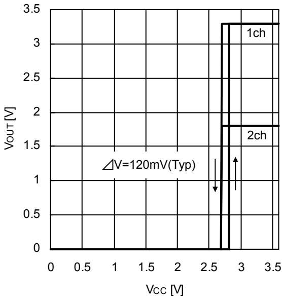
Figure.11 V CC -V OUT
