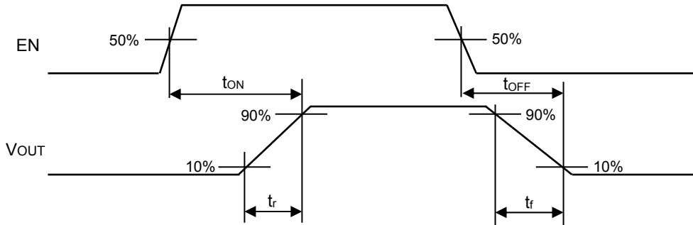
Figure.6 Timing diagram
