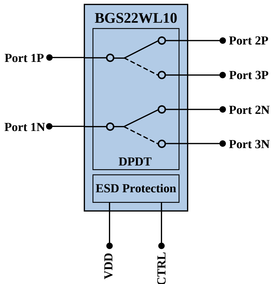
Figure 1: BGS22WL10 block diagram
