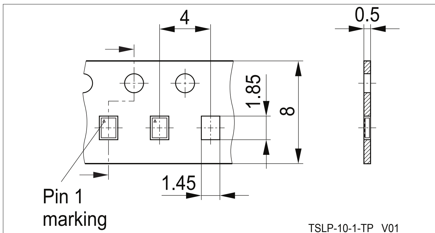
Figure 5: Tape and Reel Dimensions for TSLP-10-1
