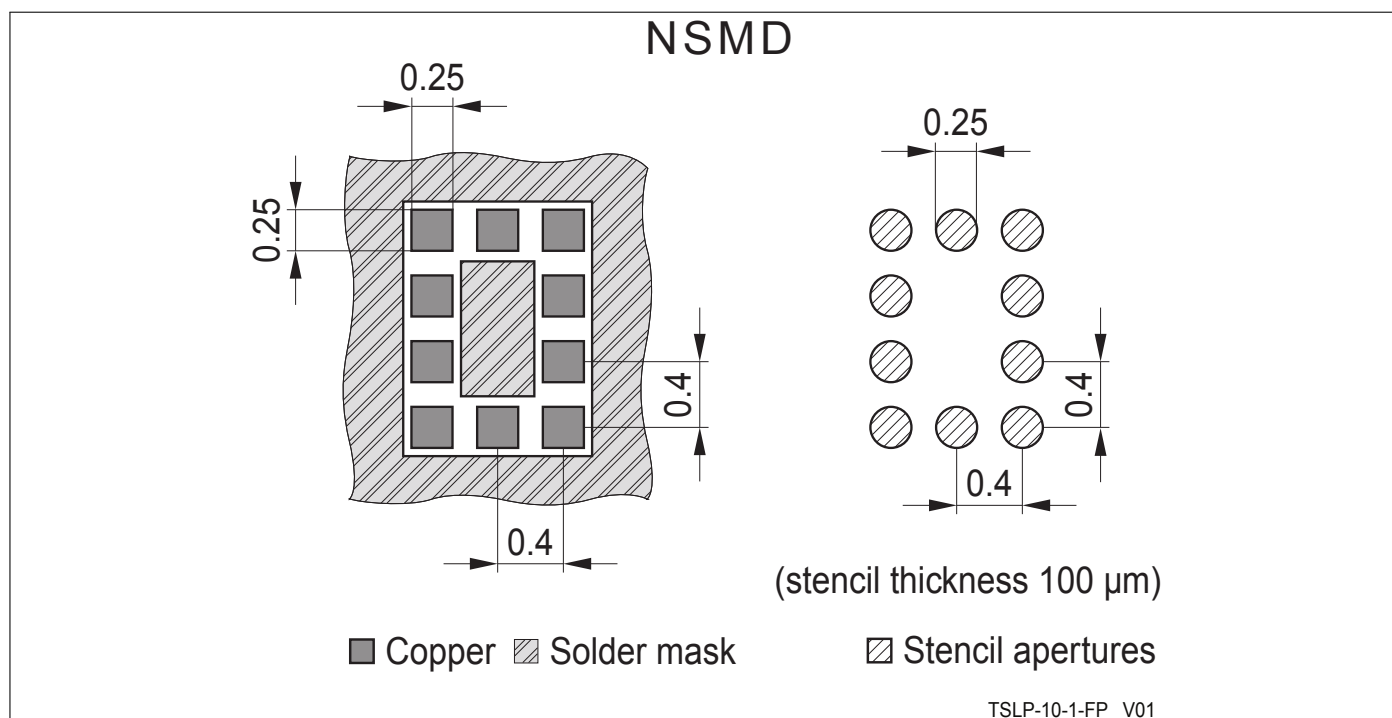
Figure 4: Footprint TSLP-10-1
