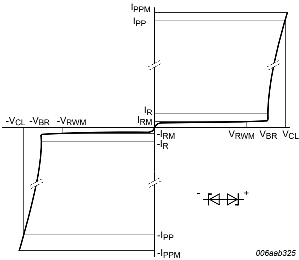
Fig. 3. V-I characteristics for a bidirectional TVS diode
