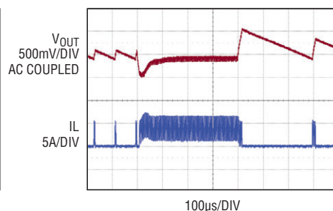
Load Step (Boost) Burst Mode Operation
