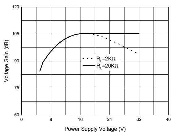
Figure 7. Voltage Gain
