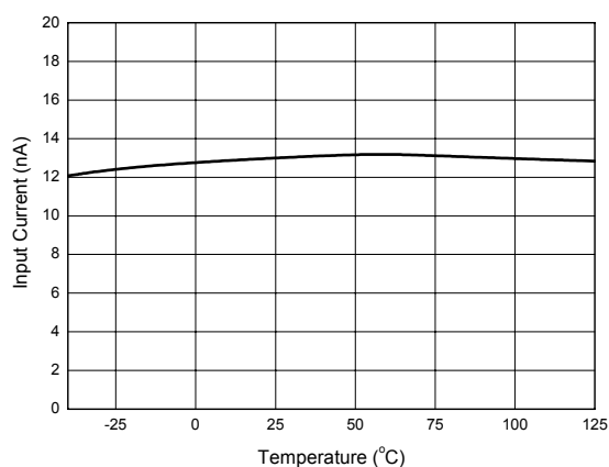
Figure 5. Input Current
