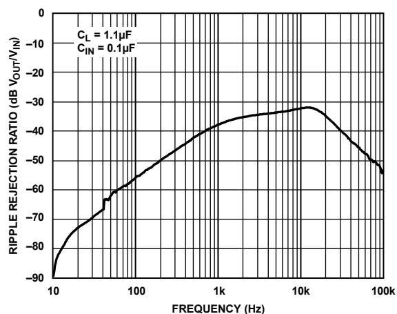
Figure 18. ADR3425 Ripple Rejection Ratio vs. Frequency
