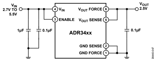
Figure 40. Basic Reference Connection
