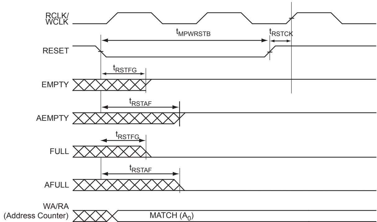
Figure 2-36 • FIFO Reset
