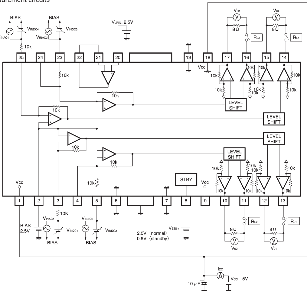
Fig.1 Driver block measurement circuit diagram
