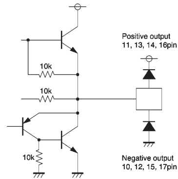
Driver output
