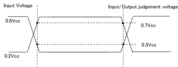
Figure 1. Input/Output judgment voltage
