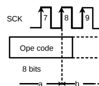
Figure 50. WREN/WRDI cancel valid timing
