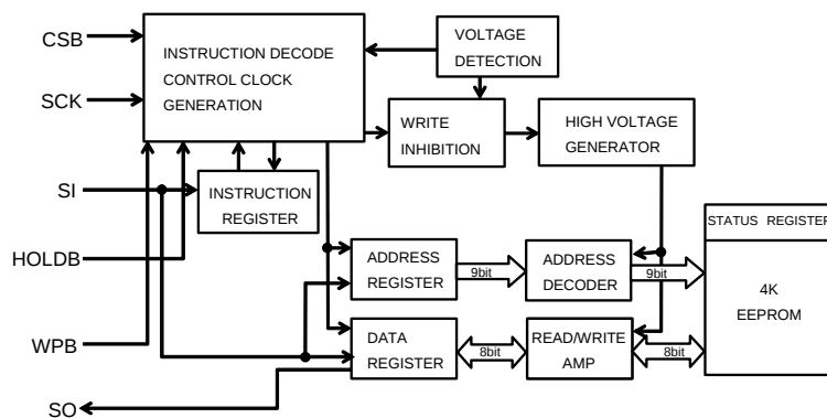
Figure 5. Block diagram
