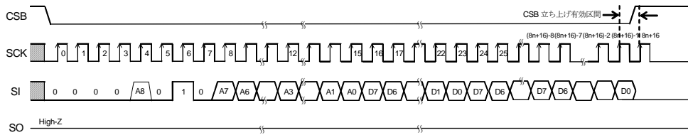
Figure 38. Write command
