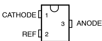
TLVH432 DBZ (SOT-23-3) PACKAGE (TOP VIEW)
