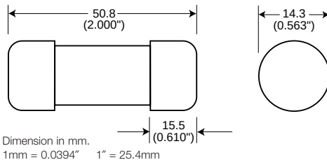
Fig. 1: 1-50 Amp Range
