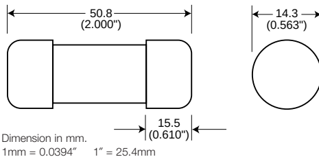
Fig. 1: 1-50 Amp Range
